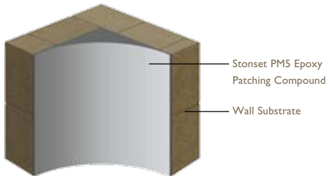
Wall to Wall or Wall to Ceiling Transition
