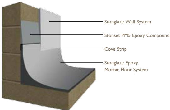
Smooth Cove Transition
