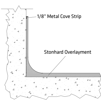
COVE BASE DETAIL WITH COVE STRIP
