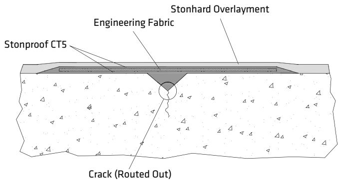
CRACK TREATMENT Stonproof CT5 with fiberglass reinforcement
